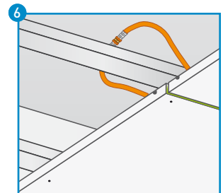
▲ Connected Modular Panels
