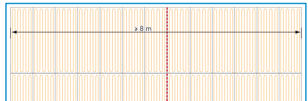
▲ Movement joint at e.g. 13xV020-100 (13x0.625 m = 8.13 m)
