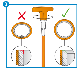
▲ Calibration and chamfering the pipe ends
