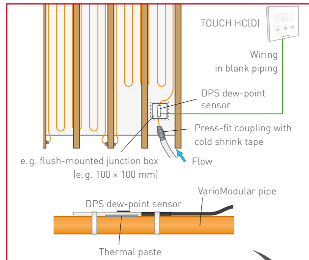
▲ Example Dew-point monitoring (cooling)
