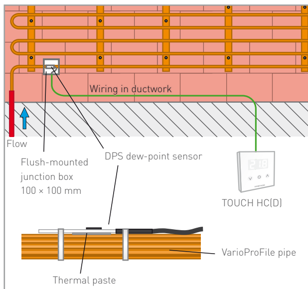
▲ Example EasyFlex wall cooling (plastered)
