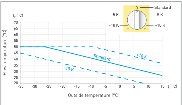
▲ Heating curve
