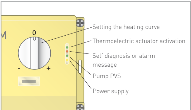
▲ Control panel
