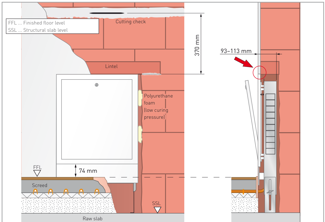
▲ Example for in-wall mounted front frame
