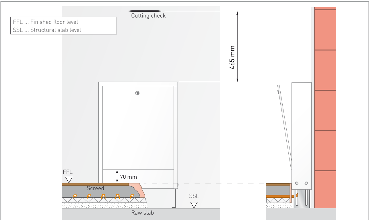
▲ Example for on-wall installation
