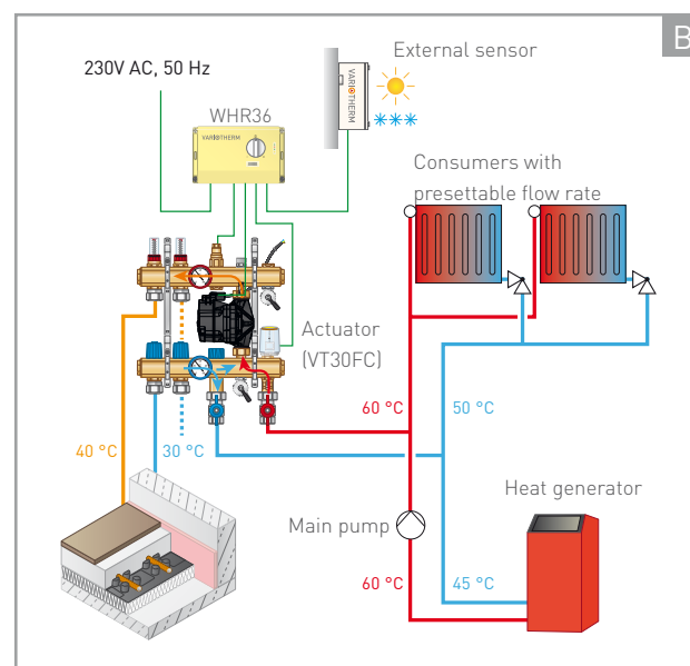
▲ Weather-guided control station
