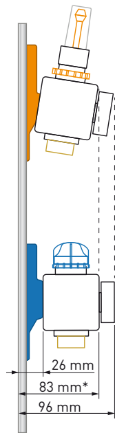
VarioManifold 5.0
