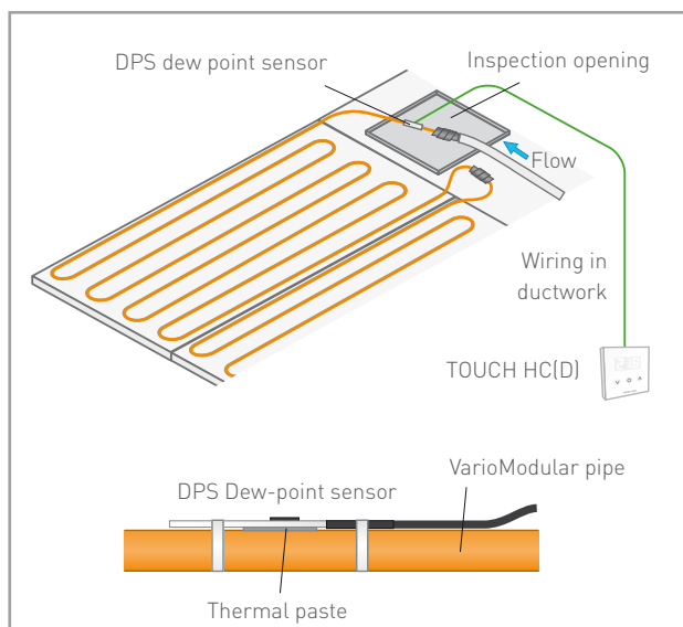
▲ Example Modular ceiling cooling (drywall)
