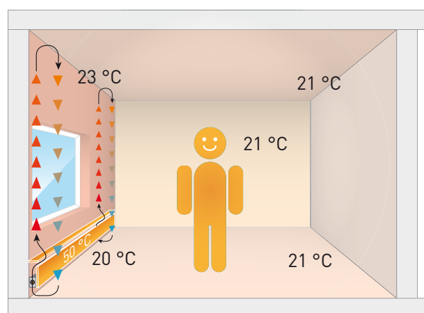
▲ Comfort with Variotherm skirting heating systems: The even heating of floor and walls creates a cosy warm envelop in the entire room. > Healthy room climate, hardly any dust stirred up, no over-heated floor, no overheated ceiling, "very cosy"
